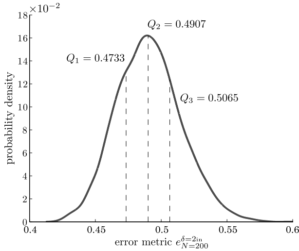
Fig. 2: Probability density function of the error metric for robot configurations randomly sampled from the ring distribution. This curve was generated by randomly sampling N = 200 robot positions from the ring distribution, calculating the value of the error metric with \delta = 2\text{in} , and repeating 100000 times. The MATLAB routine ksdensity was used to approximate the continuous probability density function from the resulting histogram. Lines for the 25 th , 50 th , and 75 th percentiles are labeled Q_1 , Q_2 , and Q_3 , respectively. In Section V, we will compare the values of the error metric achieved by the control algorithm to this probability density function to assess whether the performance is acceptable.
