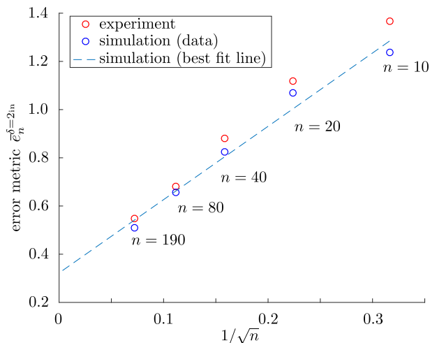
Fig. 8: Relationship between the error metric \bar{e}_n^{\delta} and number of robots n ( \delta = 2\text{in} , ring pattern). Note that the error tends toward a nonzero value as n increases. This is primarily due to the nonzero \delta , as discussed in Section III-B.
