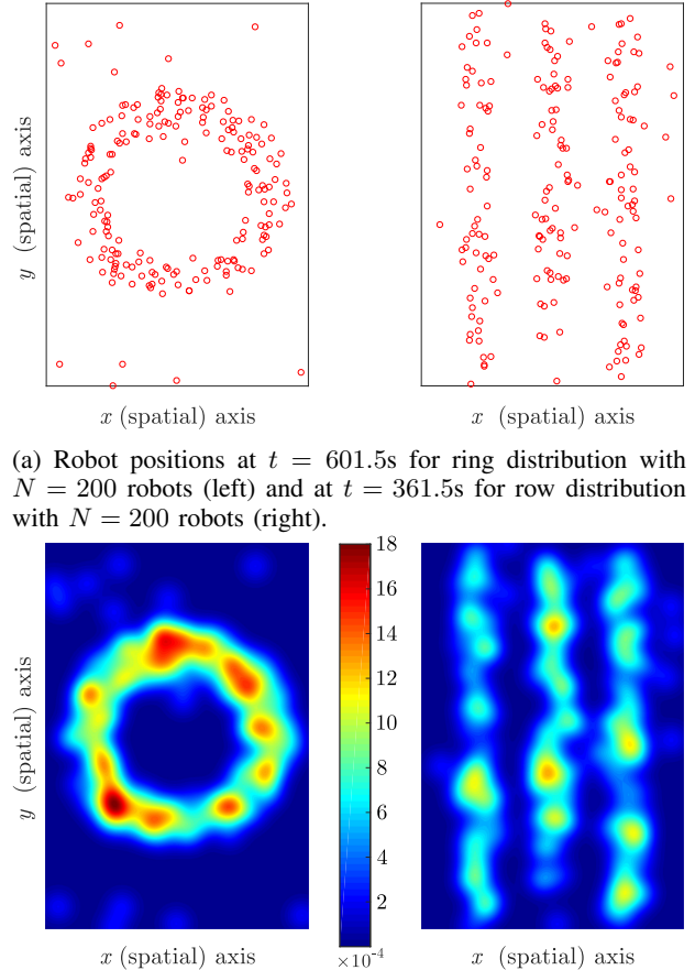
(b) Gaussian blob function \rho_{N=200}^{\delta=2in}(t = 601.5\text{s}) for ring distribution (left) and \rho_{N=200}^{\delta=2in}(t = 361.5\text{s}) for row distribution (right).
